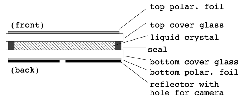
Fig. 6: Modified LC display for use with monochrome CCD or CMOS camera
