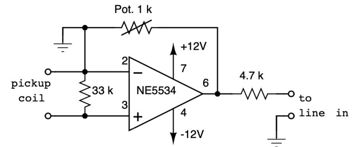
Fig. 11: VLF receiver circuit
