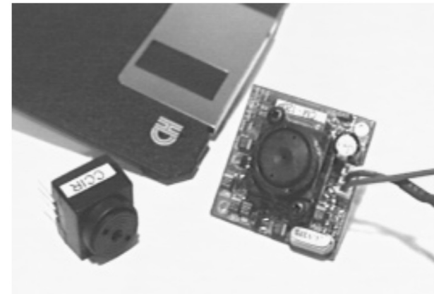
Fig. 2: CMOS (left) and CCD (right) pinhole camera
