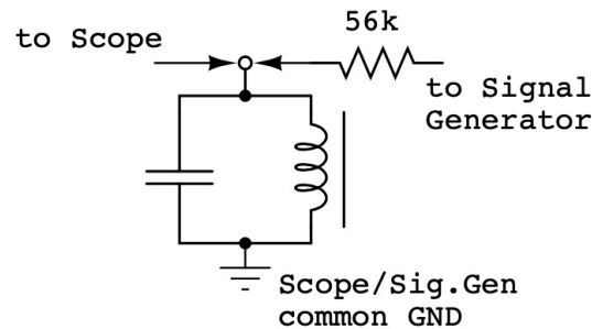
Fig. 12: Setup used for determining the resonant frequency
