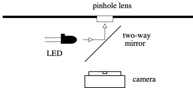
Fig. 4: Camera hidden behind an operating control light
