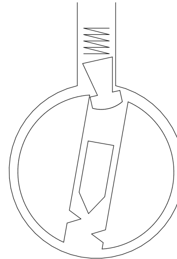
Figure 9.7: Mushroom, spool, and serrated driver pins
