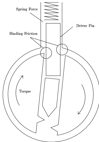
Figure 5.2: Binding in the pin-column model
