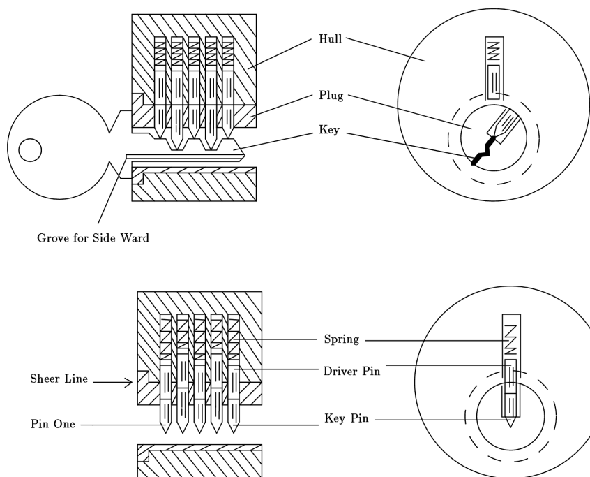
Figure 2.1: Workings of pin tumbler locks
