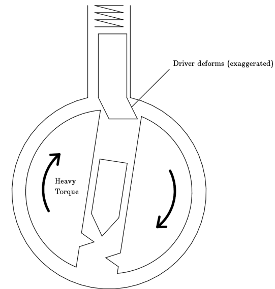
Figure 9.2: Driver pin false set by elastic deformation
