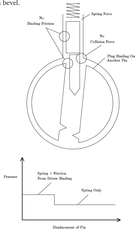
Figure 9.3: Driver pin wider than key pin
