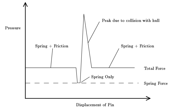
Figure 5.5: Pressure required to move pins
