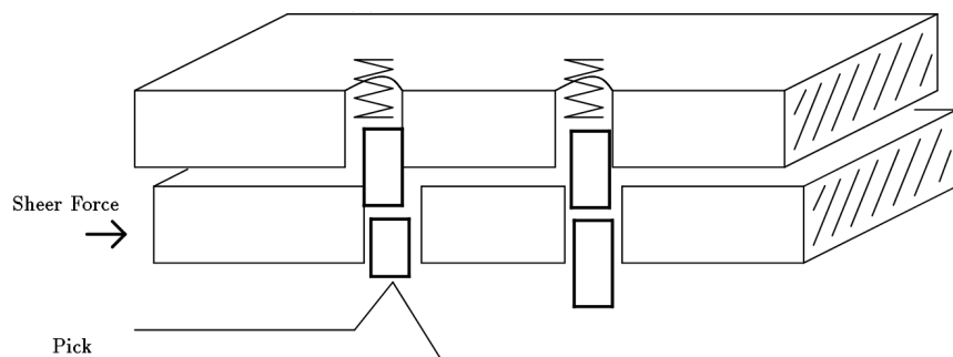
Figure 4.2: (b) Pick lifts the binding pin
