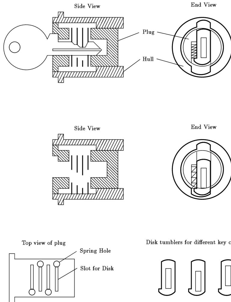
Figure 9.10: Workings of a disk tumber lock
