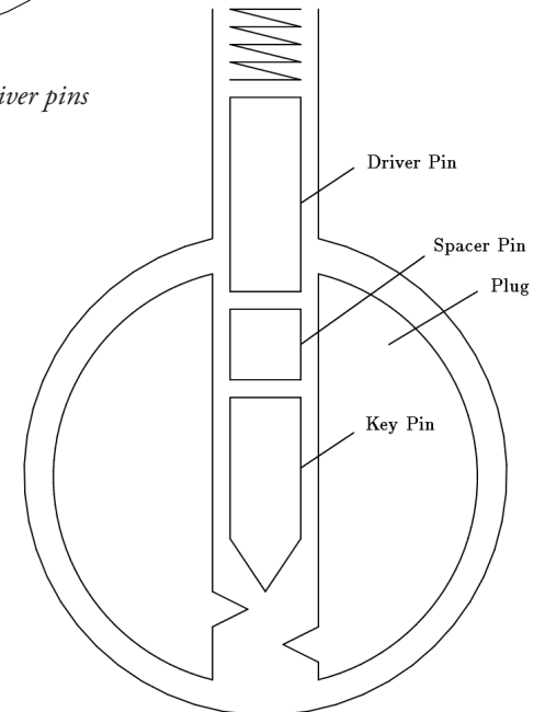
Figure 9.8: Spacer pins for master keying
